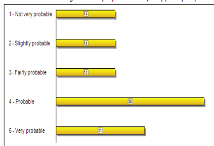
Raw data: histogram of simple probabilities (dolat) (All experts)
