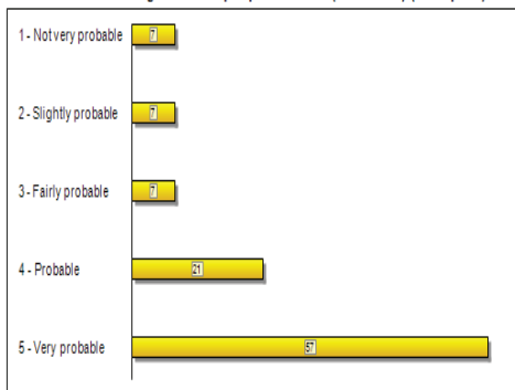
Raw data: histogram of simple probabilities (arzech din) (All experts)
